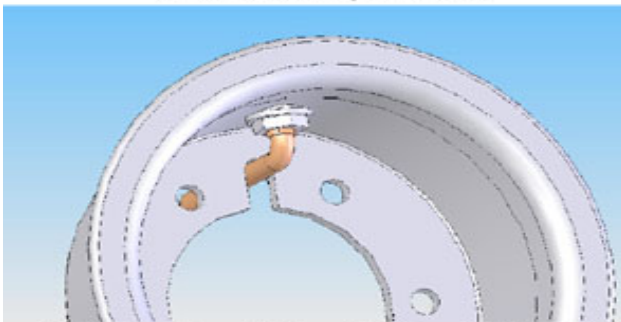
Install Valve Stem Washer (dimple up) & Valve Nut
