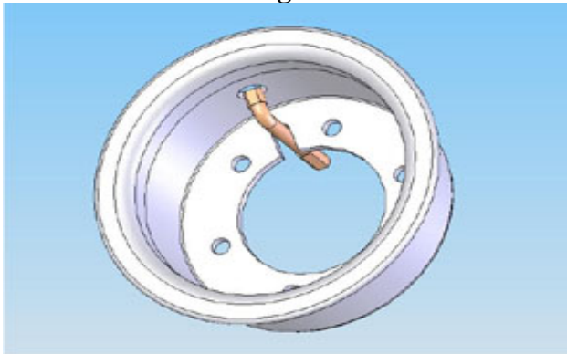
Install Valve Stem Thru Hole in Back Half and Align With Slot
