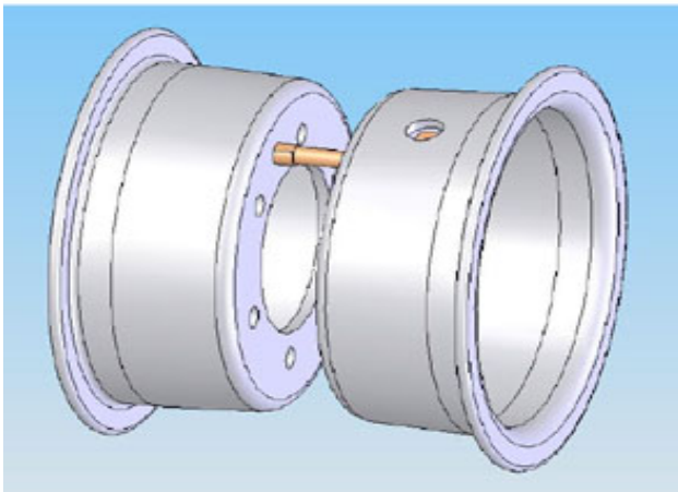
Insert Stem into Valve Hole in Valve Half & Align Bolt Holes
